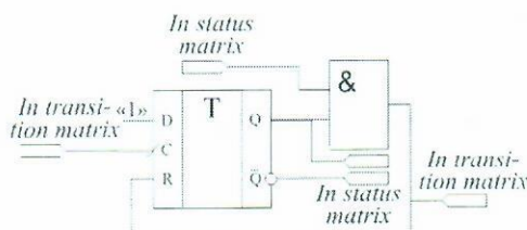
Fig. 4. Interconnection of a status and transition
