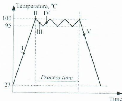
Fig. 7. Used control process
