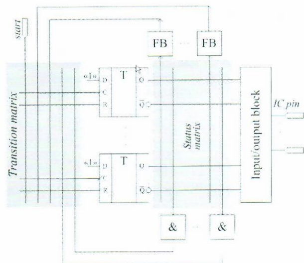
Fig. 6. Offered PLD architecture
